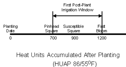
Figure 1. Early season cotton plant development as a function of heat units, and general window for timing of the first post-plant irrigation.
