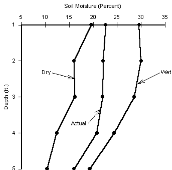
Figure 2. Soil moisture content at the time of the first post-plant irrigation (Pima clay loam, Marana, AZ).
