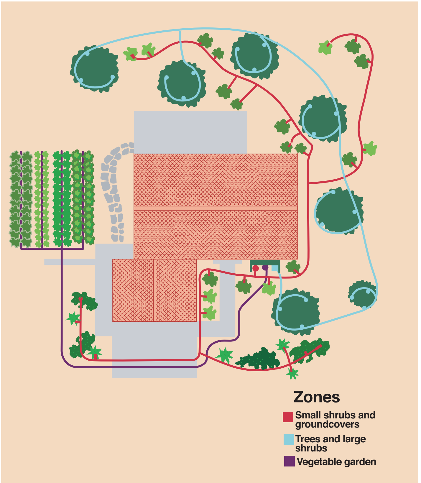
This drip irrigation system has three valves for plants with different water needs. Vegetables are watered most frequently with drip tape installed in the bed. Small shrubs and groundcovers have individual drip emitters with low flow rates (0.5 or 1 gph). Trees and large shrubs have multiple emitters with higher flow rates (4 gph) and are watered deep and infrequent.
